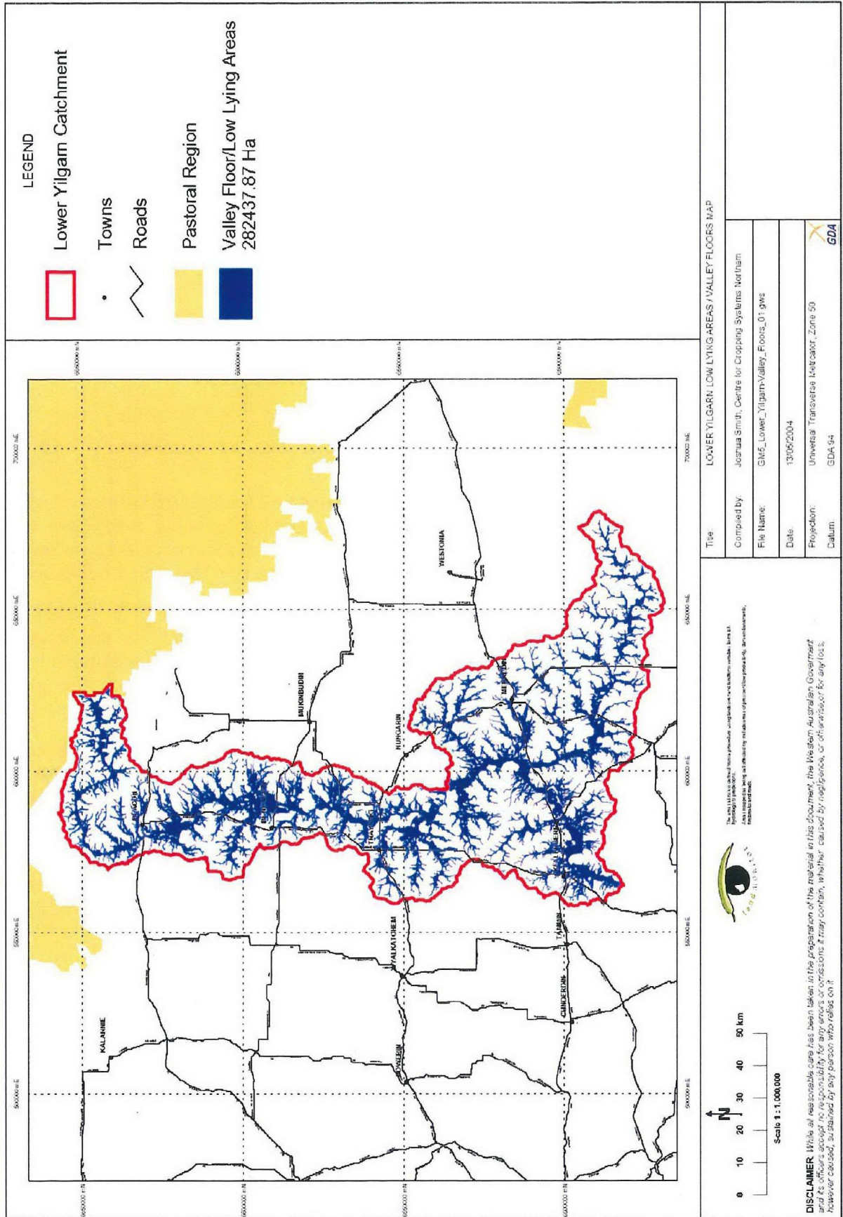
Figure 3.2: Valley floors
