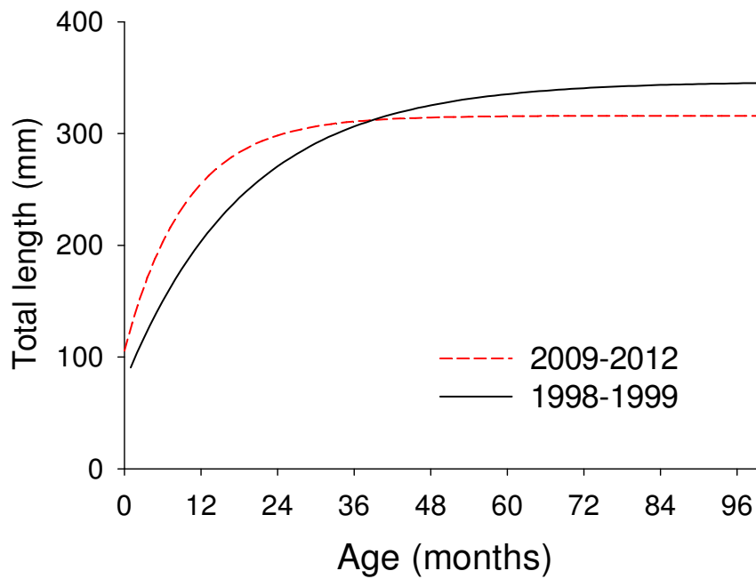
Figure 2.2. Comparison of von Bertalanffy growth curves for Hyporhamphus melanochir in the West Coast Bioregion (WCB) (sexes combined), estimated from samples collected in 1998-1999 (Jones et al. 2002) and in 2009-2012 (Section 3).
