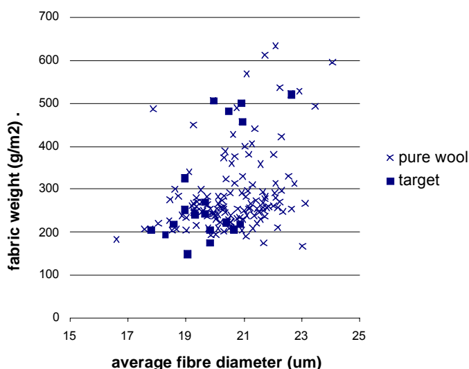
Figure 1: Average fibre diameter and fabric weight for 148 pure wool fabrics, target fabrics are identified.
